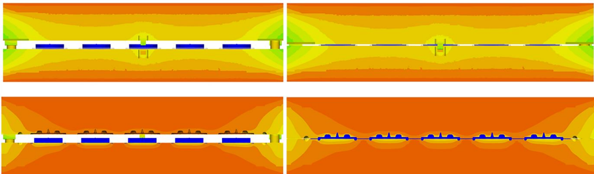
Bild 1 – The view of the mold when opening: left, when closing: right. Thermal influences in the mold seen from the outside: above, from the center: below.
